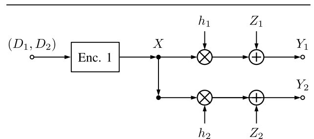
Fig. 7. Two-user BC with AWGN.
