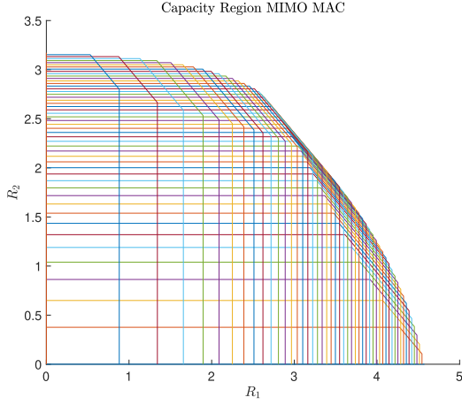
Fig. 11. MIMO MAC capacity region for 2 \times 2 channel.
